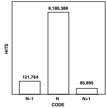
TPC 3. "Grounded-Input" Histogram (Input Span = 2 V p-p)
