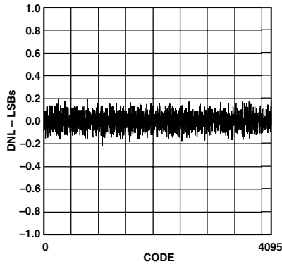
TPC 10. Typical DNL
