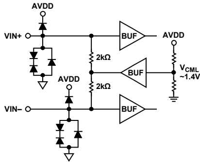
Figure 34. Analog Inputs ( V_{CM} = \sim 1.4 V )
