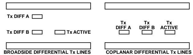
Figure 80. Broadside vs. Coplanar Differential Stripline Routing Techniques
