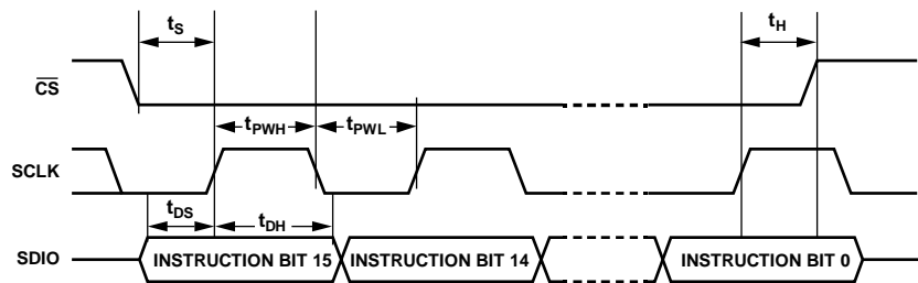
Figure 25. Timing Diagram for Serial Port Register Write
