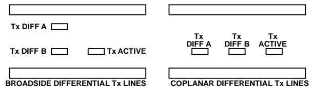
Figure 60. Broadside vs. Coplanar Differential Stripline Routing Techniques
