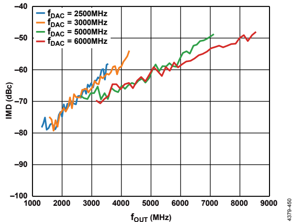
Figure 38. IMD vs. f_{OUT} over f_{DAC}
