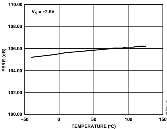
Figure 19. Large Signal PSSR vs. Temperature
