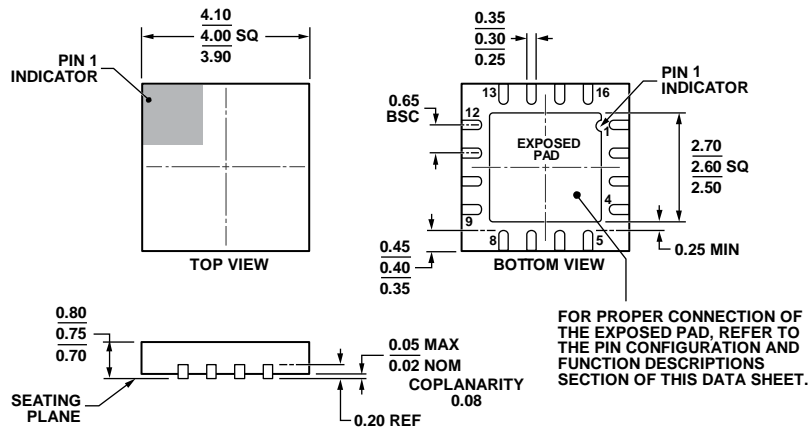
Figure 61. 16-Lead Lead Frame Chip Scale Package [LFCSF_WQ] 4 mm x 4mm Body, Very Very Thin Quad (CP-16-17) Dimensions shown in millimeters
