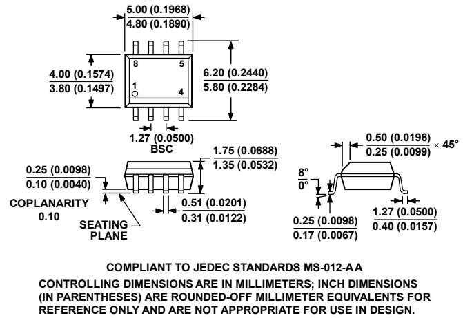
Figure 72. 8-Lead Standard Small Outline Package [SOIC_N] Narrow Body (R-8) Dimensions shown in millimeters and (inches)
