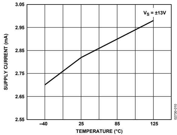
Figure 10. Supply Current vs. Temperature at ±13 V
