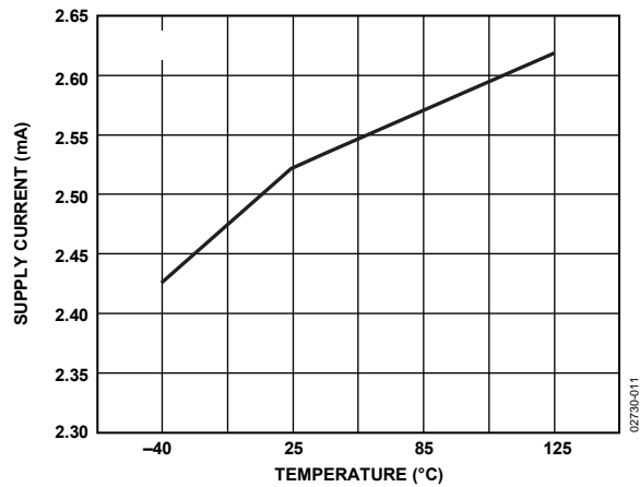
Figure 11. Supply Current vs. Temperature at ±5 V
