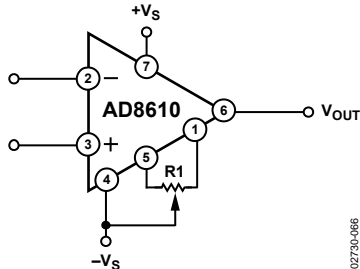
Figure 66. Offset Voltage Nulling Circuit
