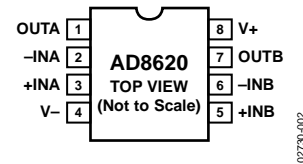
Figure 2. AD8620 8-Lead SOIC
