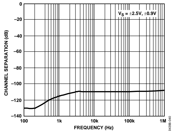
Figure 40. Channel Separation
