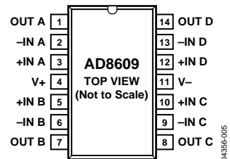
Figure 5. 14-Lead SOIC_N (R Suffix)
