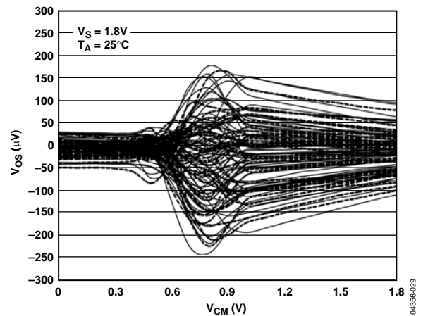
Figure 29. Input Offset Voltage vs. Common-Mode Voltage
