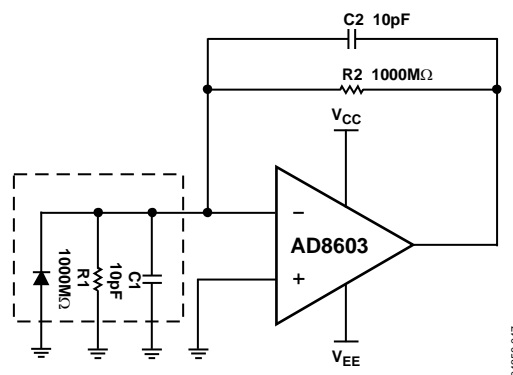
Figure 47. Photodiode Circuit
