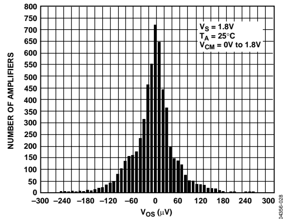
Figure 28. Vos Distribution
