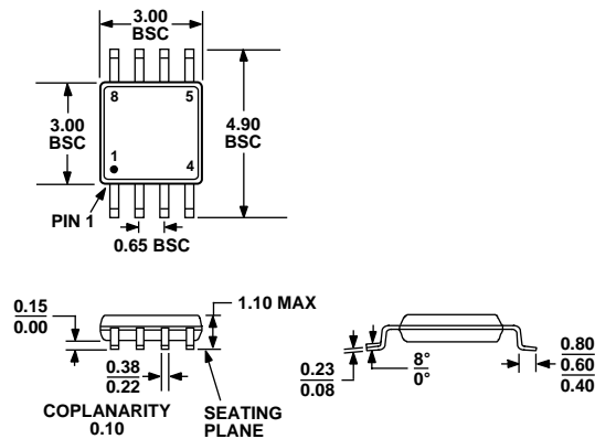
Figure 50. 8-Lead Mini Small Outline Package [MSOP] (RM-8)
