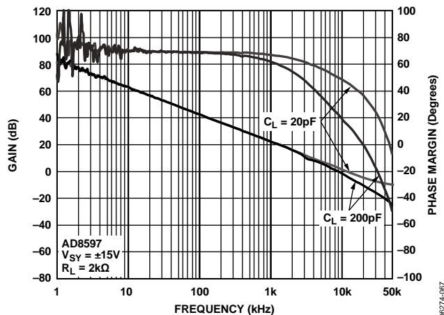
Figure 33. Gain and Phase vs. Frequency
