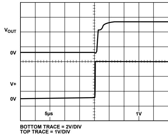
Figure 61. AD857x Output Behavior on Power-Up
