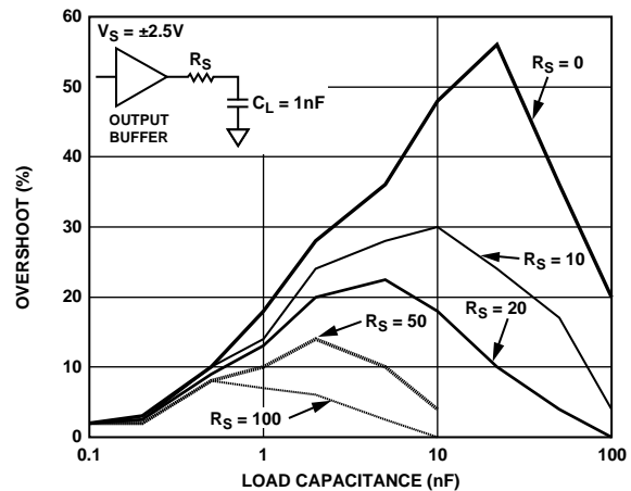
Figure 57. Positive Overshoot Graph vs. C_L
