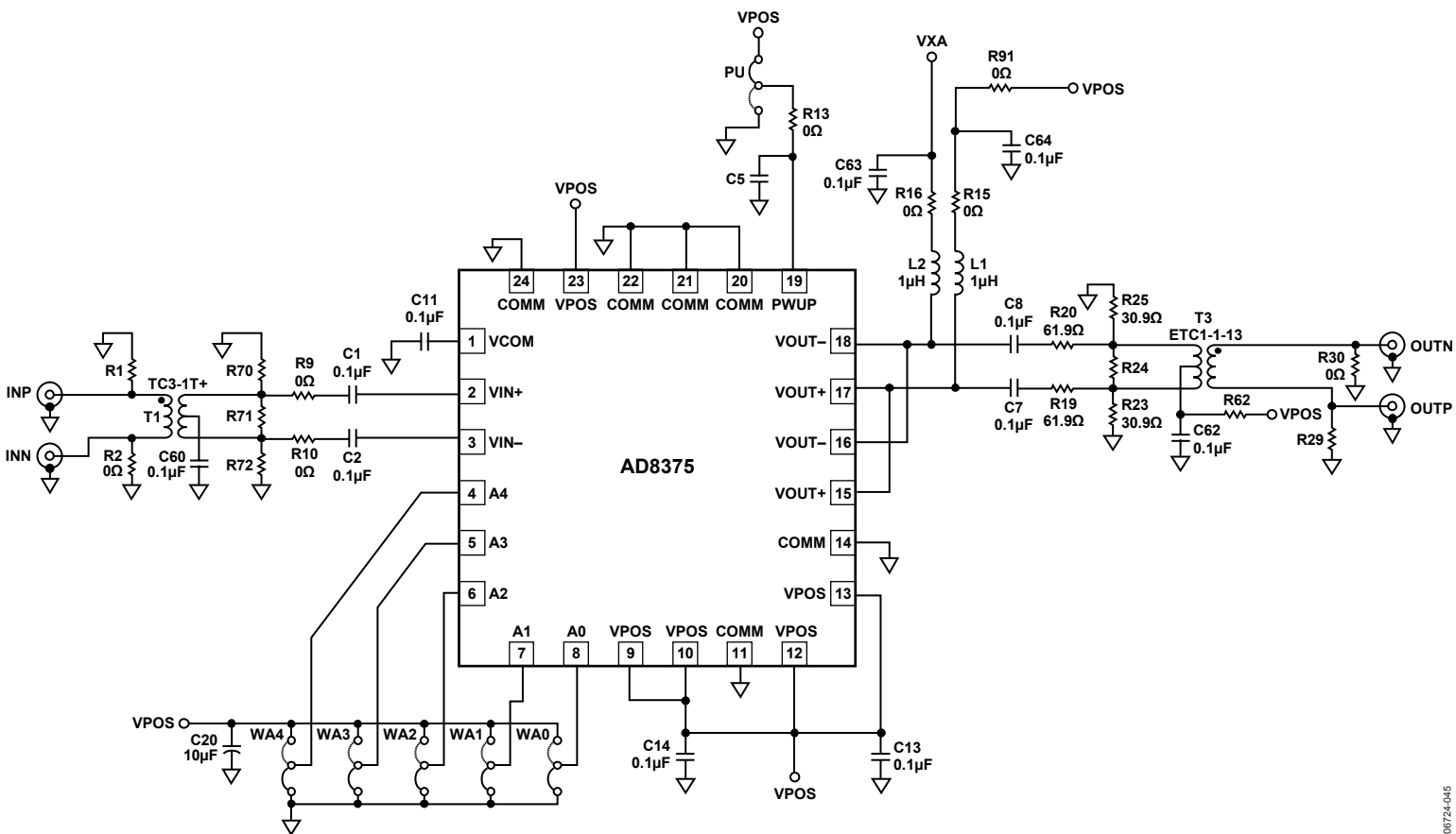
Figure 46. AD8375 Evaluation Board Schematic
