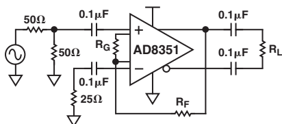
Figure 5. Single-Ended Application
