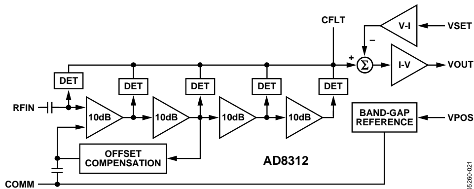
Figure 21. Block Schematic
