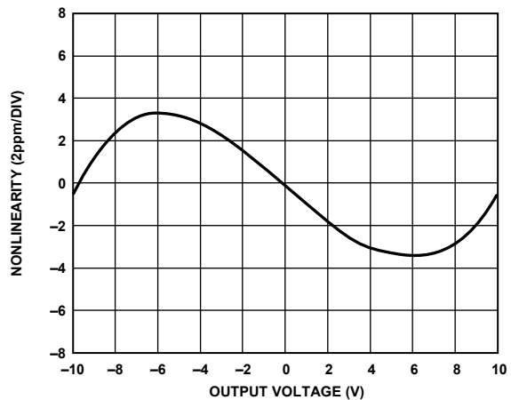
Figure 27. Gain Nonlinearity, V_S = \pm 15\text{ V} , R_L \geq 2\text{ k}\Omega
