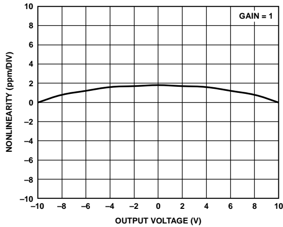
Figure 36. Gain Nonlinearity, G = 1 , R_L = 10\text{ k}\Omega
