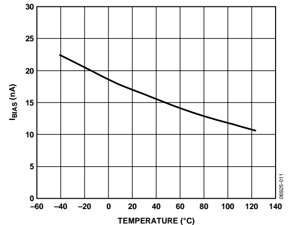
Figure 7. I_{\text{BIAS}} vs. Temperature
