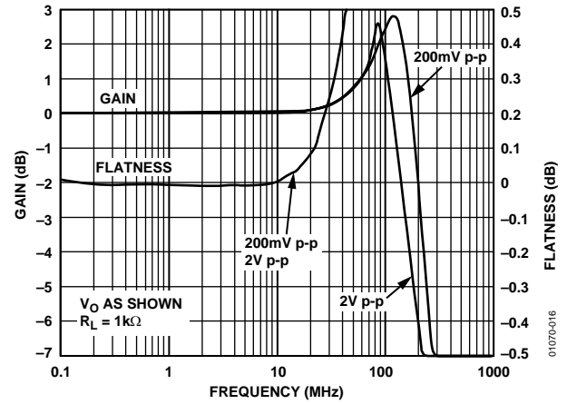
Figure 11. AD8115 Frequency Response, R_L = 1\ k\Omega
