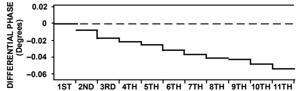
Figure 22. Differential Gain and Phase Error, G = 2 , NTSC Input Signal, R_L = 1k\Omega , V_S = 5V
