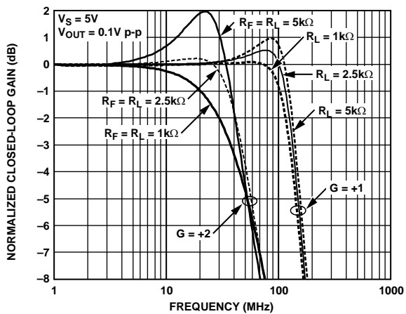
Figure 55. Frequency Response for Various Feedback/Load Resistances
