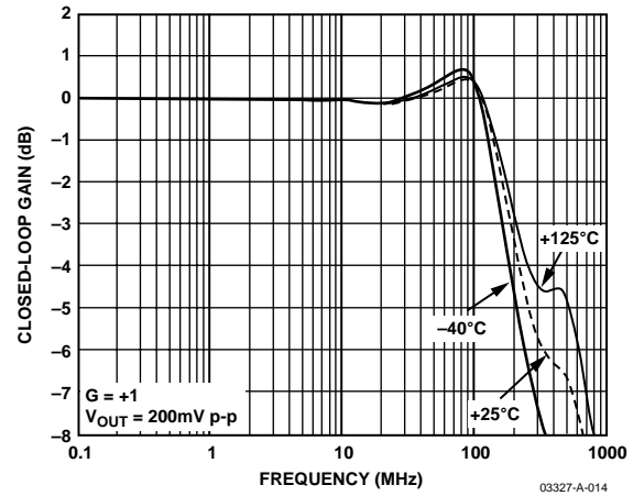
Figure 15. AD8028 Small Signal Frequency Response vs. Temperature
