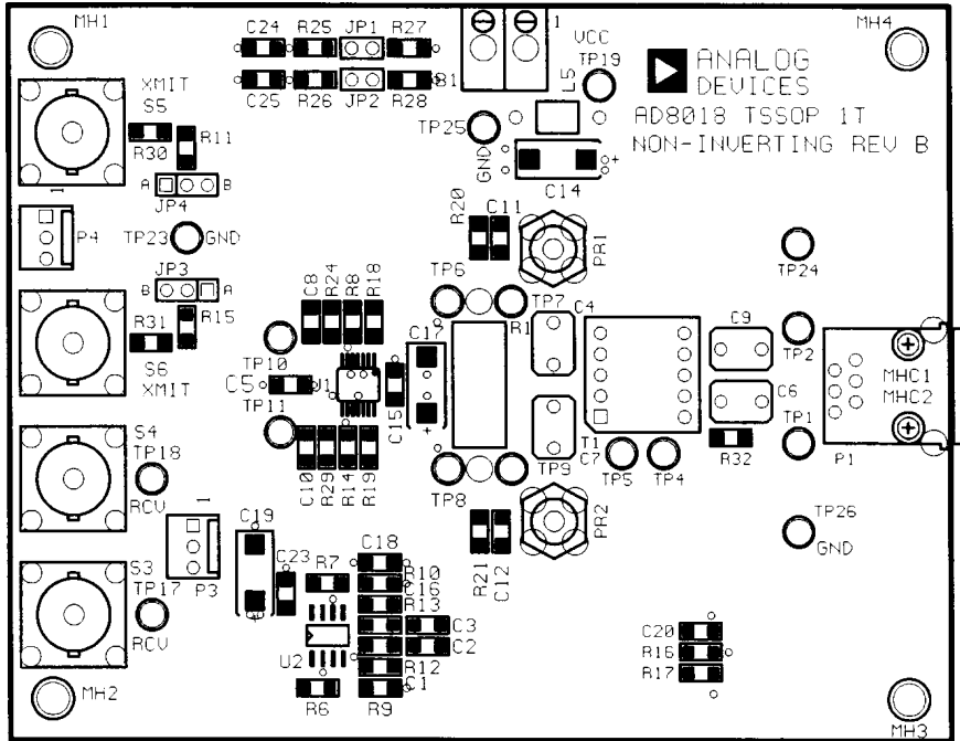
Figure 13. Assembly—Primary Side
