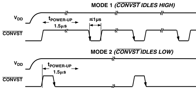
Figure 12. Power-Up Times
