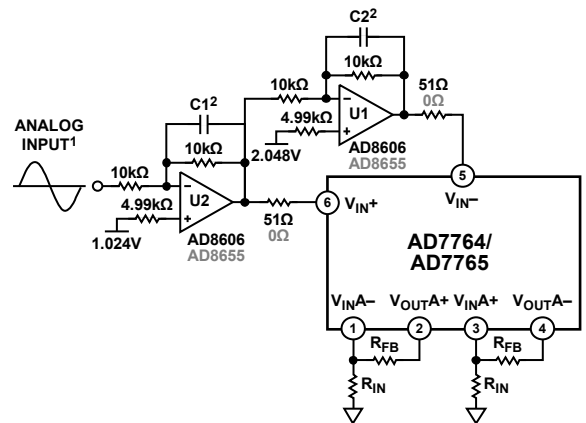
Figure 34. Driving the AD7765 Modulator Inputs Directly from a Single-Ended Source (On-Board Differential Amplifier Powered Down)
