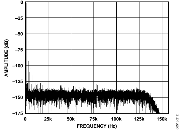
Figure 9. Low Power Mode, FFT, 1 kHz, -0.5\text{ dB} Input Tone, 64\times Decimation Rate
