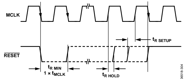
Figure 46. RESET Timing Synchronous to MCLK
