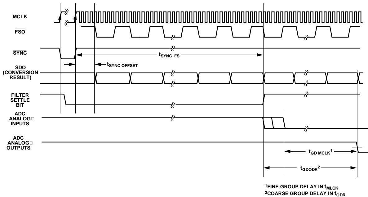
Figure 34. AD7764 Digital Filtering; Response to SYNC, Settling Time, and Group Delay
