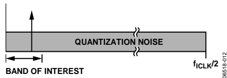
Figure 30. \Sigma - \Delta ADC, Quantization Noise
