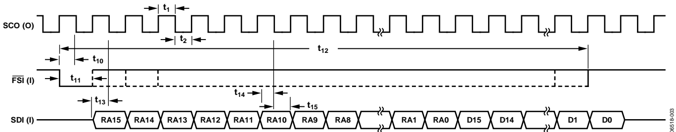
Figure 3. Register Write Timing Diagram
