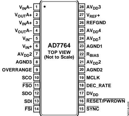
Figure 5. Pin Configuration
