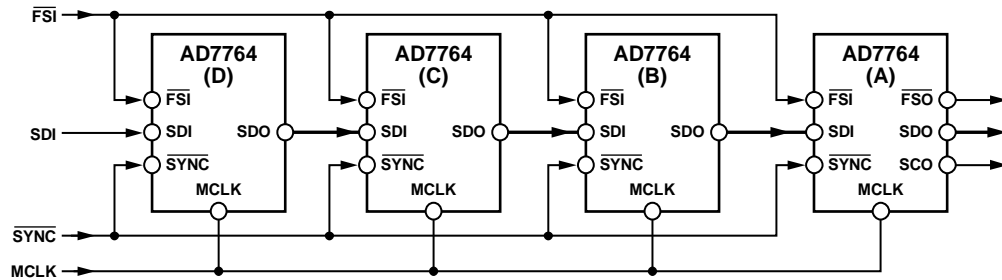
Figure 49. Writing to an AD7764 Daisy-Chain Configuration
