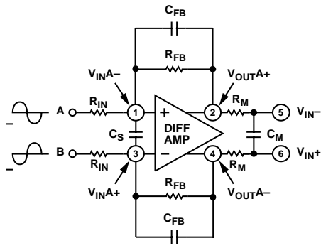
Figure 37. Differential Amplifier Configuration
