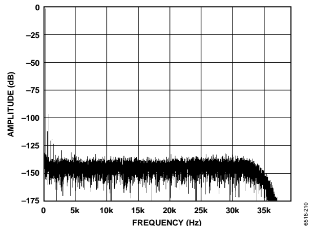
Figure 11. Low Power Mode, FFT, 1 kHz, -0.5\text{ dB} Input Tone, 256\times Decimation Rate
