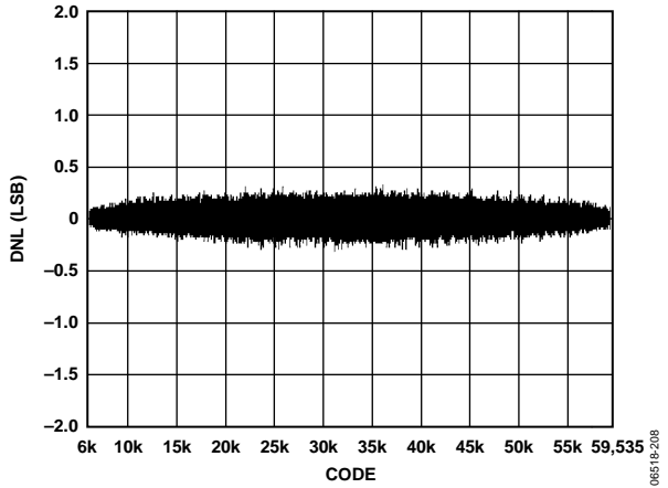
Figure 24. DNL Plot
