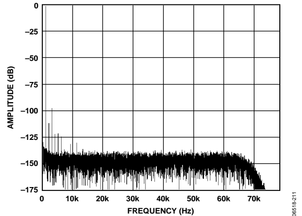
Figure 10. Low Power Mode, FFT, 1 kHz, -0.5\text{ dB} Input Tone, 128\times Decimation Rate
