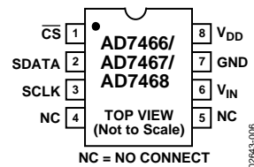
Figure 5. MSOP Pin Configuration
