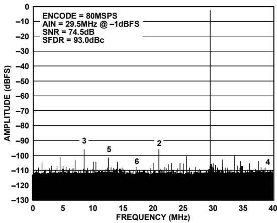
Figure 6. Single Tone @ 29.5 MHz
