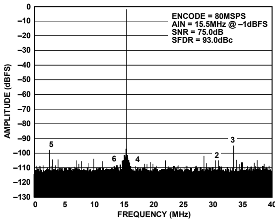
Figure 5. Single Tone @ 15.5 MHz
