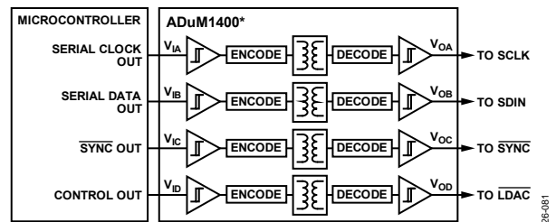
Figure 88. Isolated Interface
