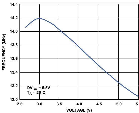
Figure 70. Internal Oscillator Frequency vs. D VCC Supply Voltage
