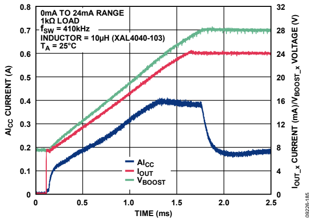
Figure 83. I_{CC} Current vs. Time for 24 mA Slew with External 51 k \Omega Compensation Resistor
