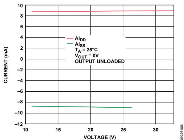
Figure 67. A IDD /A ISS vs. A VDD /A VSS
