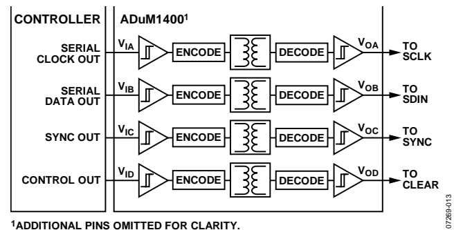
Figure 57. Isolated Interface
