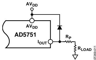
Figure 55. Output Transient Voltage Protection
