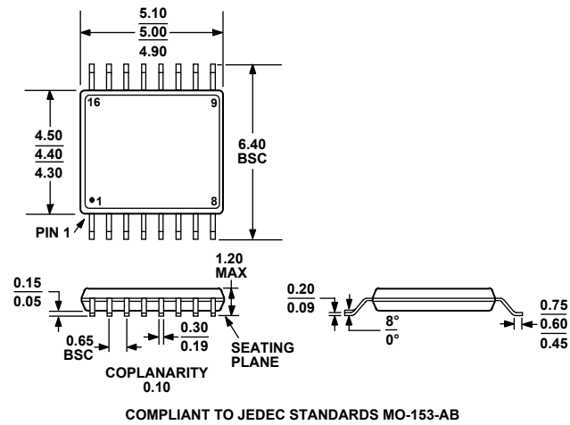
COMPLIANT TO JEDEC STANDARDS MO-153-AB Figure 52. 16-Lead Thin Shrink Small Outline Package [TSSOP] (RU-16) Dimensions shown in millimeters
