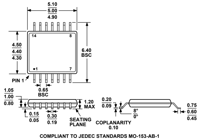
COMPLIANT TO JEDEC STANDARDS MO-153-AB-1 Figure 51. 14-Lead Thin Shrink Small Outline Package [TSSOP] (RU-14) Dimensions shown in millimeters
