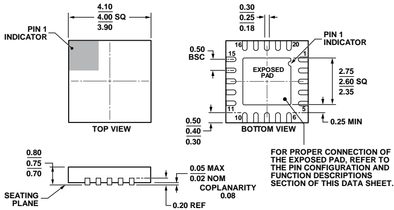
Figure 74. 20-Lead Lead Frame Chip Scale Package [LFCSP_WQ]
