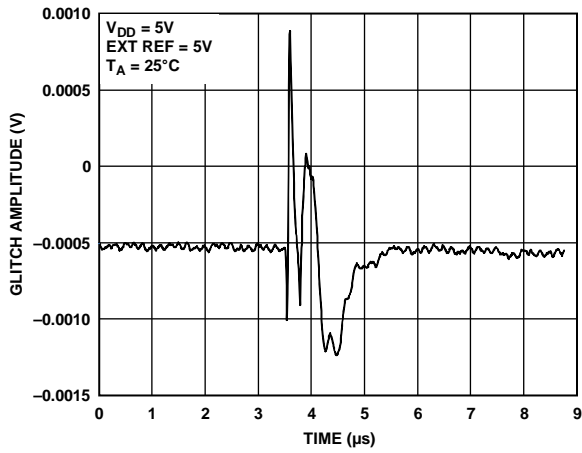
Figure 43. Analog Crosstalk
