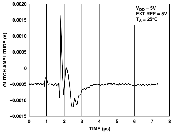
Figure 44. DAC-to-DAC Crosstalk
