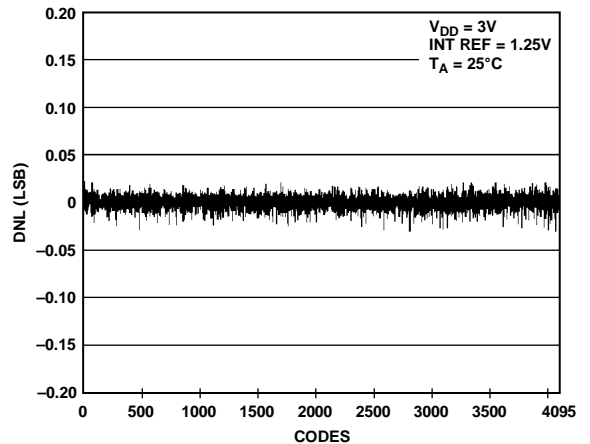
Figure 24. DNL AD5628-1
