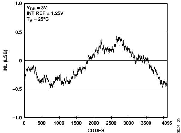
Figure 21. INL AD5628-1
