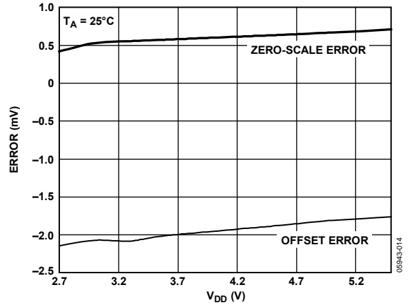
Figure 15. Zero-Scale Error and Offset Error vs. Supply
