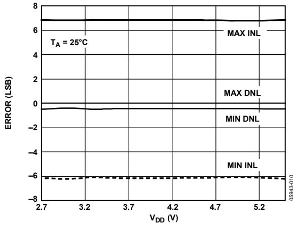
Figure 11. INL and DNL Error vs. Supply
