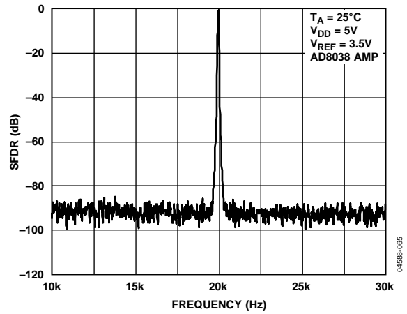
Figure 32. Narrow-Band SFDR, f_{OUT} = 20\text{ kHz} , Clock = 1 MHz
