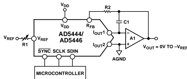
Figure 38. Unipolar Operation
