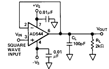
Figure 23c. Unity Gain Follower
