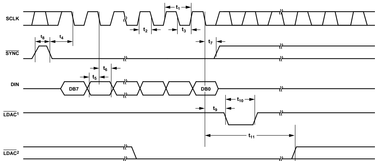
Figure 2. Timing Diagram
