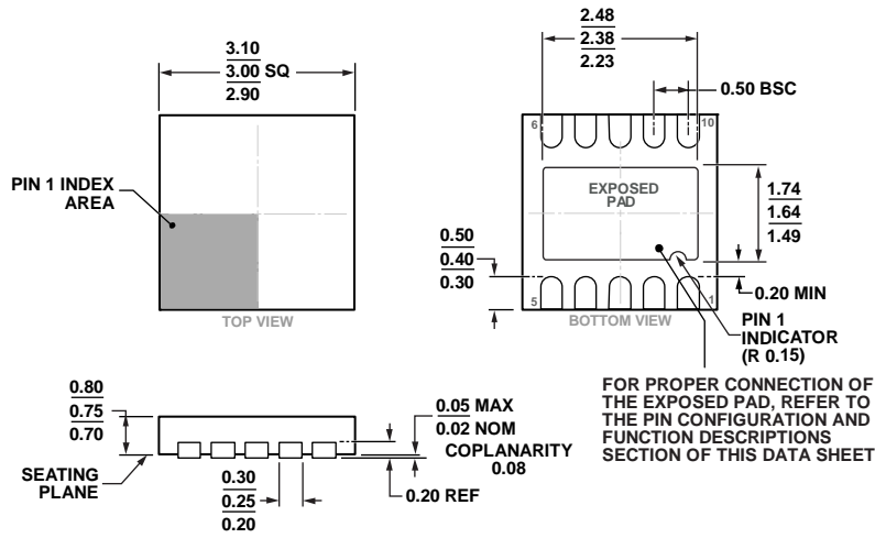
Figure 50. 10-Lead Frame Chip Scale Package [LF CSP] (CP-10-9) 3 mm x 3mm Body, Very Thin, Dual Lead Dimensions shown in millimeters
