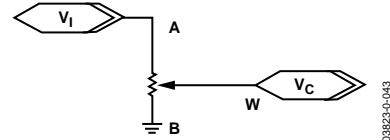
Figure 43. Potentiometer Mode Configuration
