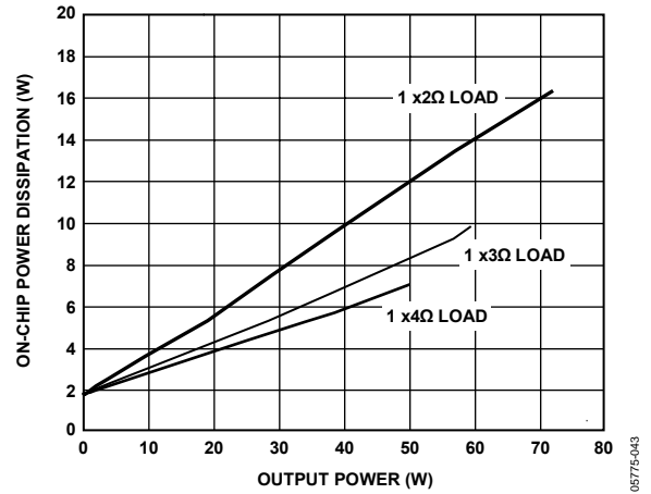
Figure 42. On-Chip Power Dissipation vs. Output Power, Mono Mode, PVDD = 18 V
