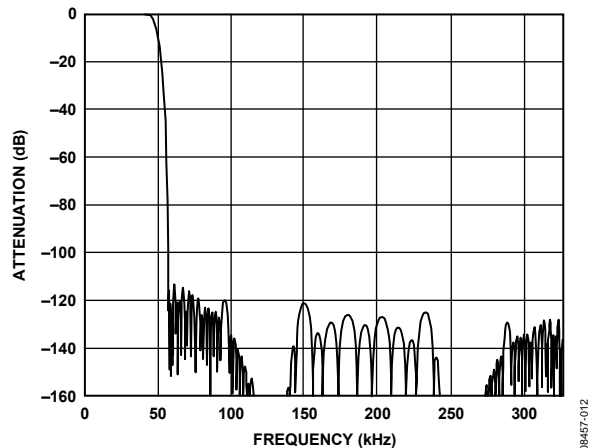
Figure 12. Complete Response, 4x Mode, 96 kHz Sample Rate
