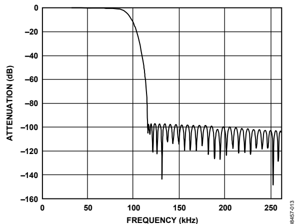
Figure 13. Complete Response, 2x Mode, 192 kHz Sample Rate
