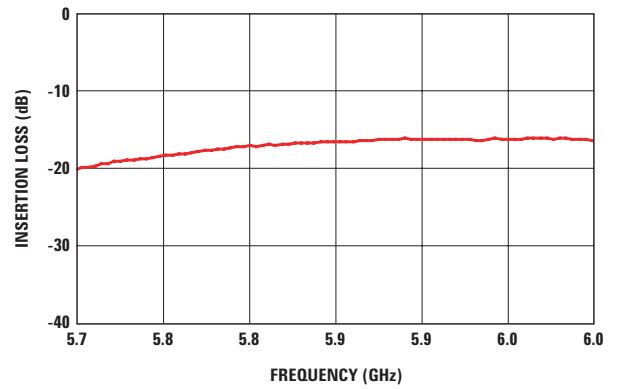
Figure 8. Tx third harmonic rejection
