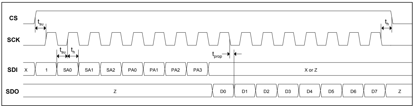
Figure 10: Read Operation
