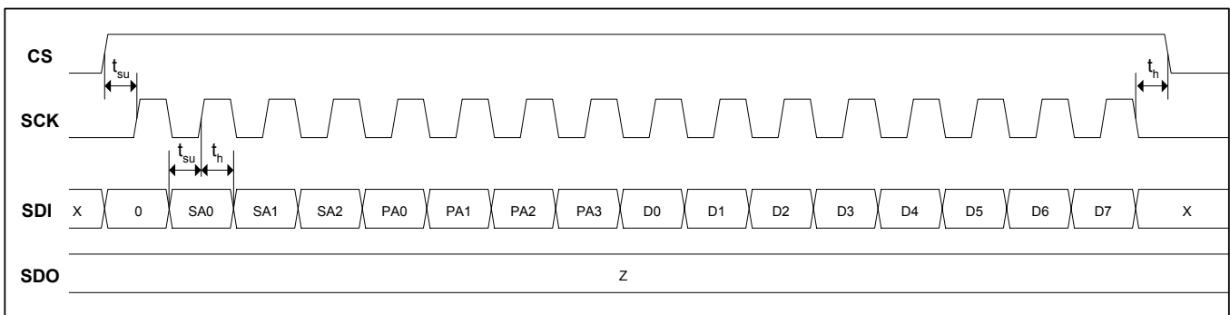
Figure 11: Write Operation
