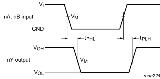
Fig. 8. The data input (nA or nB) to output (nY) propagation delays
