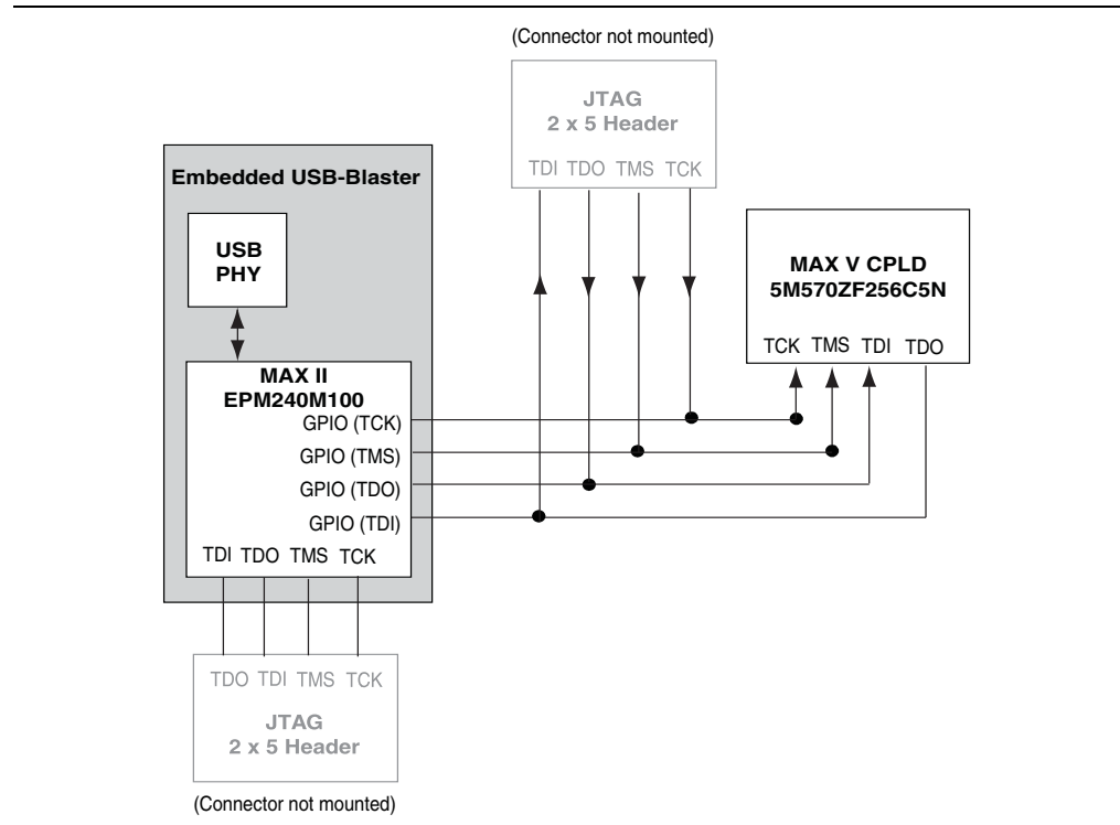
Figure 2–3. JTAG Chain
