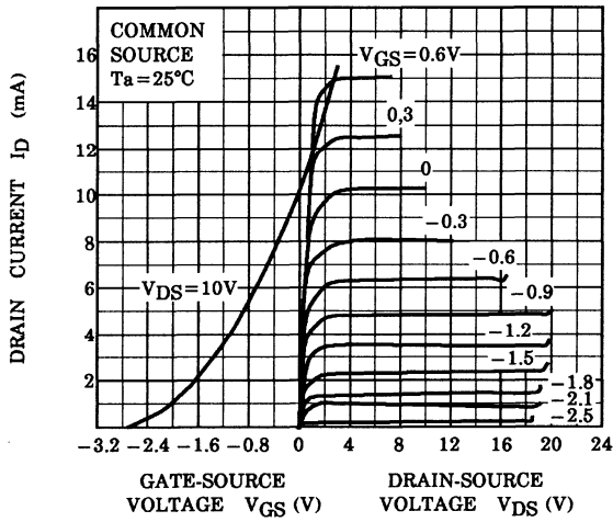
STATIC CHARACTERISTICS
