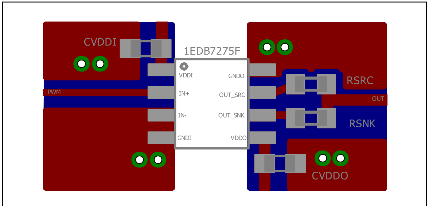
Figure 11 Layout recommendation
